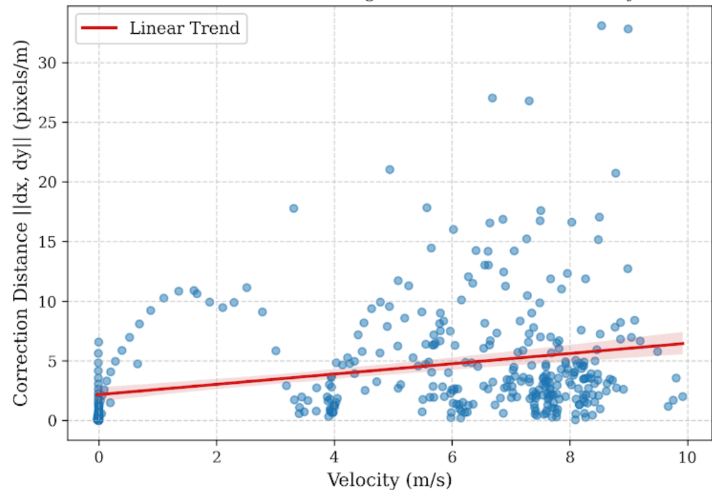
A: EKF Correction Magnitude vs. Vehicle Velocity
