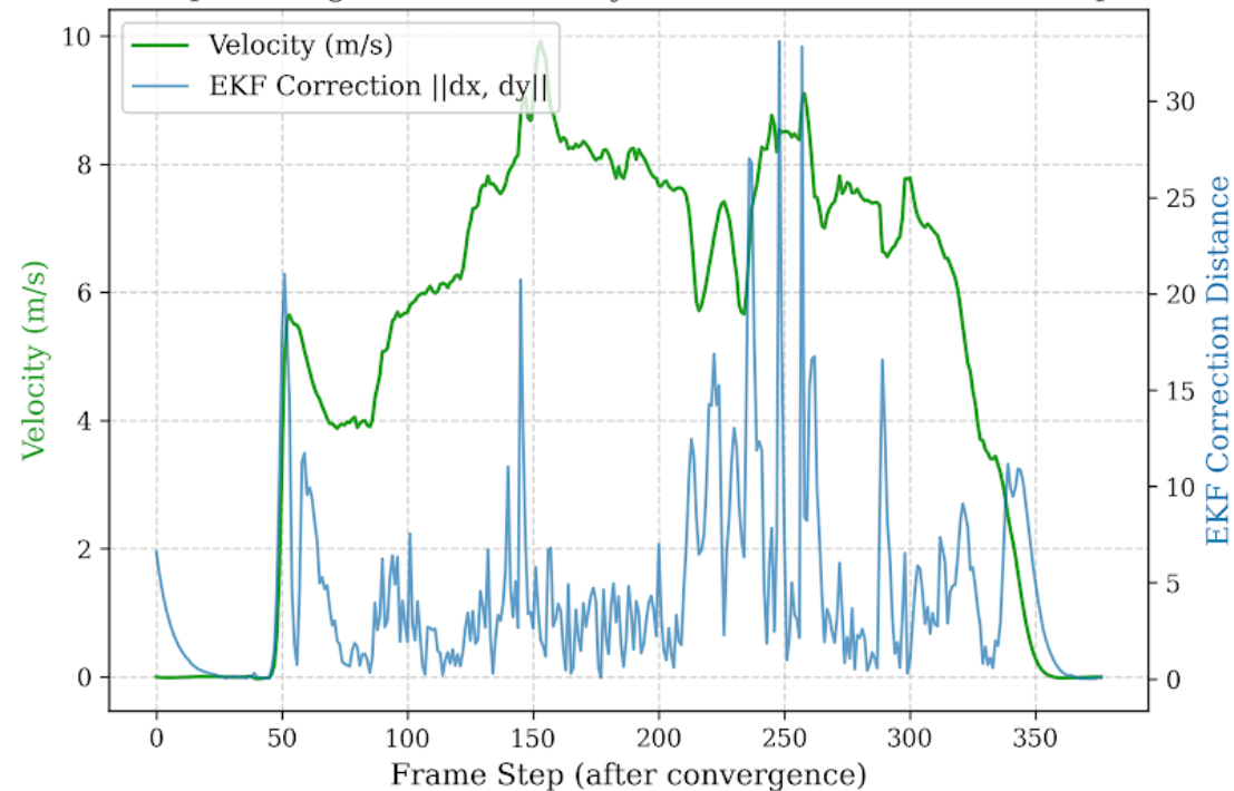
C: Temporal Alignment of Velocity Peaks and EKF Correction Spikes
