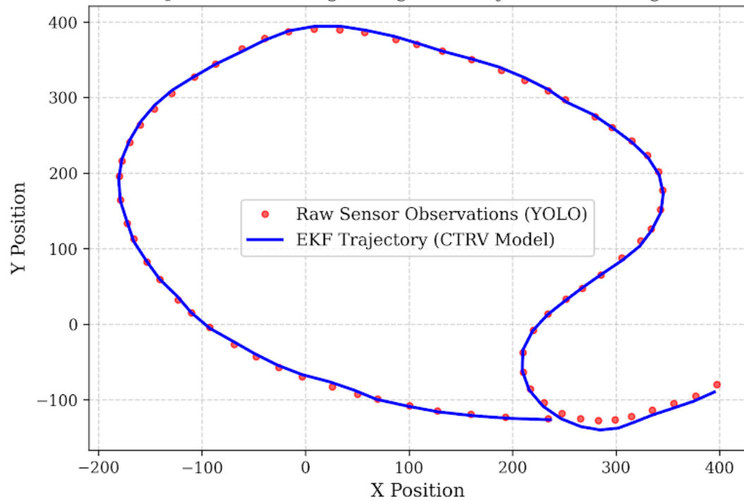
D: Spatial Smoothing in High-Velocity Maneuver Segment
